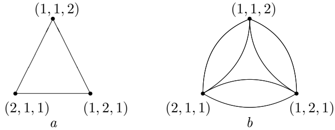
FIGURE 5. Dual complex of x^8 + y^8 + z^8 + x^2 y^2 z^2 .
